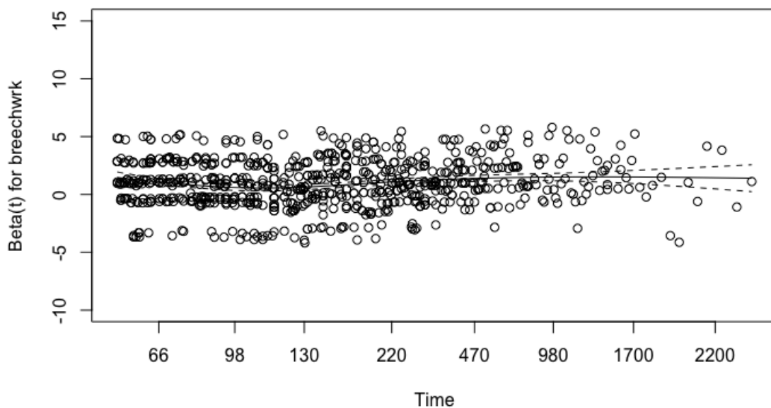
Figure 7 Testing the proportional hazards assumption for the breach wrinkle score model (summer rainfall environment): plot of scaled Schoenfeld residuals against transformed survival time
